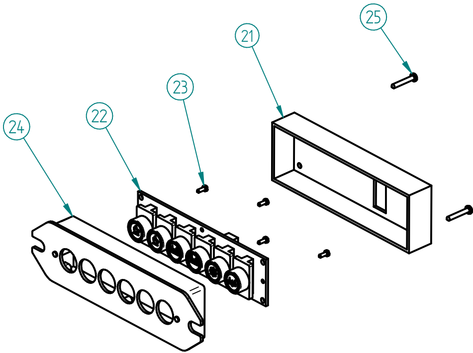
5 - 7.0.07.0109 - TECLADO 6T Ø16 CONJ. COMPASS Ø16 6T KEYBOARD ASS. COMPASS
