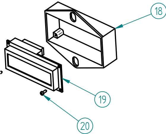
5 - 7.0.07.0109 - TECLADO 6T Ø16 CONJ. COMPASS Ø16 6T KEYBOARD ASS. COMPASS
