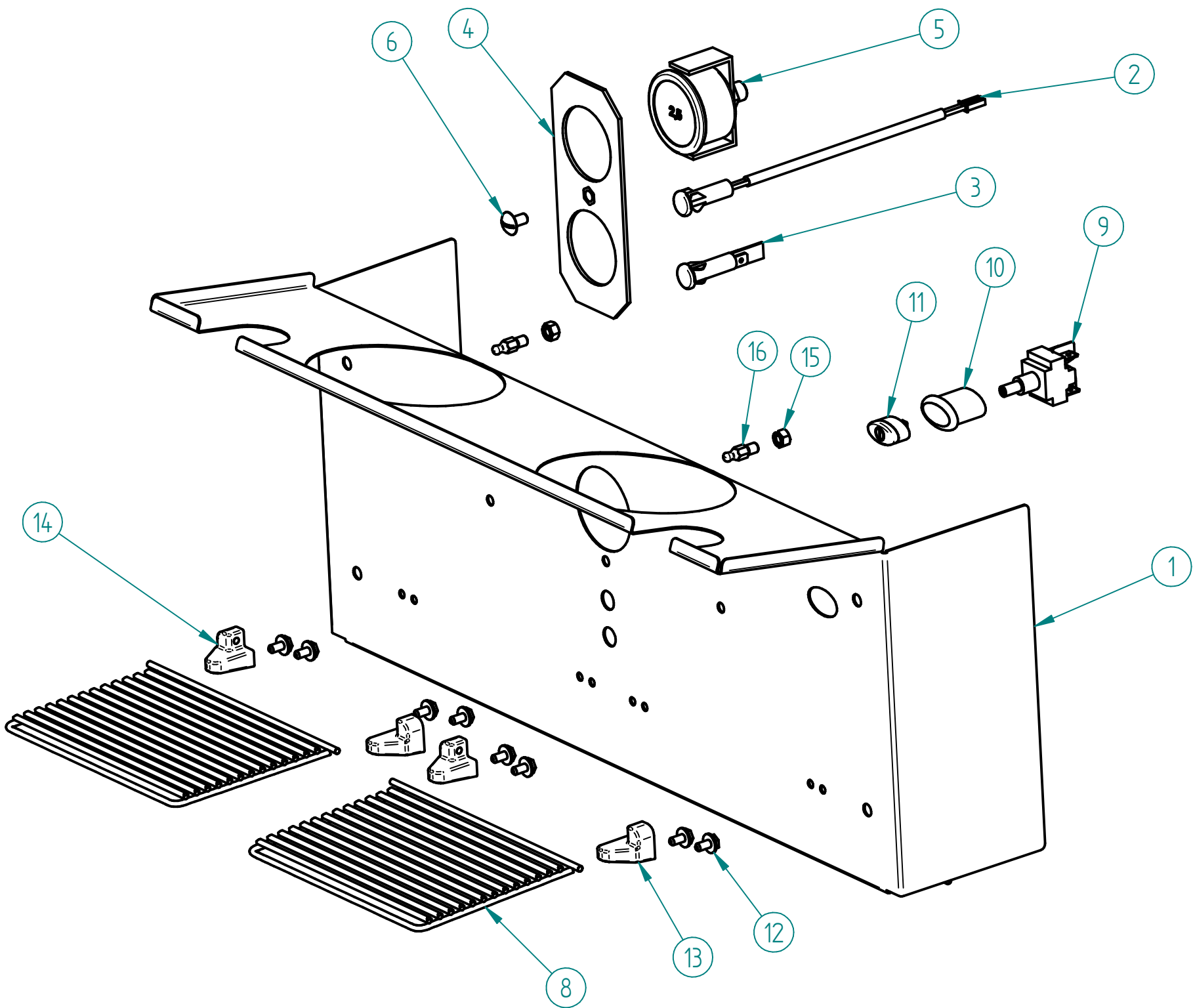
14 – PAINEL FRONTAL CONJ. COMPACT/2PB 14 – FRONT PANEL COMPACT/2PB
