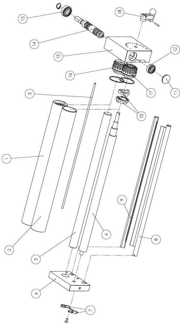
Figure 2 - Lower roller unit
