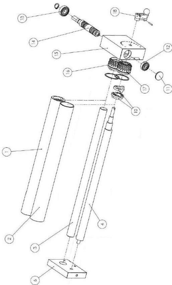
Figure 3 - Upper roller unit
