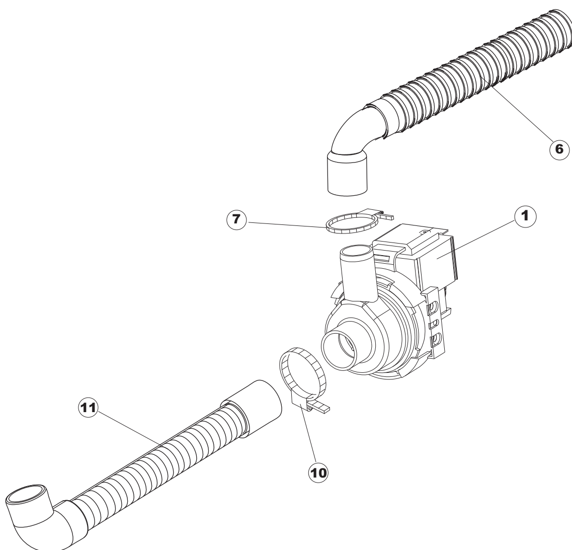
Drain pump(Optional)
