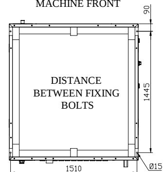
MACHINE FRONT
