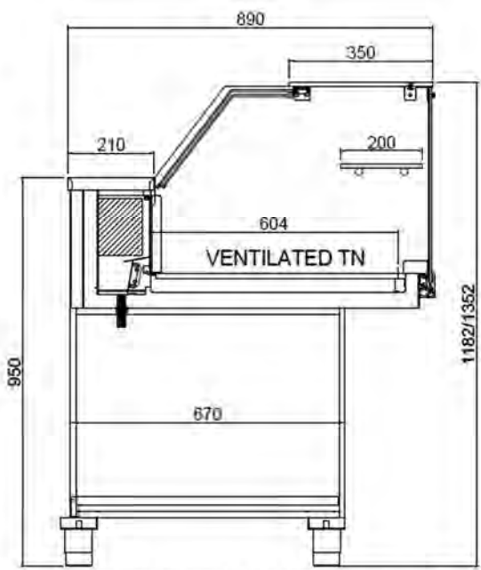
SECTION OF LOWER GLASS VENTILATED TN
