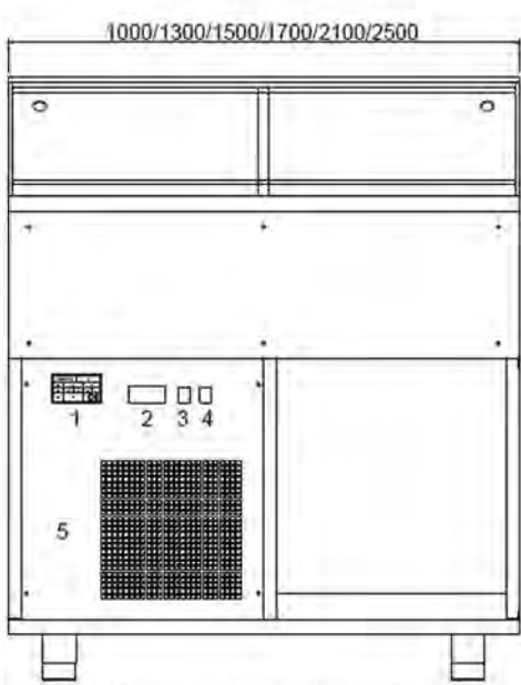
VIEW OF OPERATOR'S SIDE
