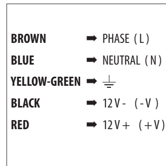
D3. Connect the new power supply as above
