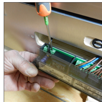
H4. Reconnect the probe to the thermoregulator
