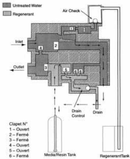
Position C3 - Rinçage lent
