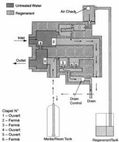
Position C2 - Aspiration
