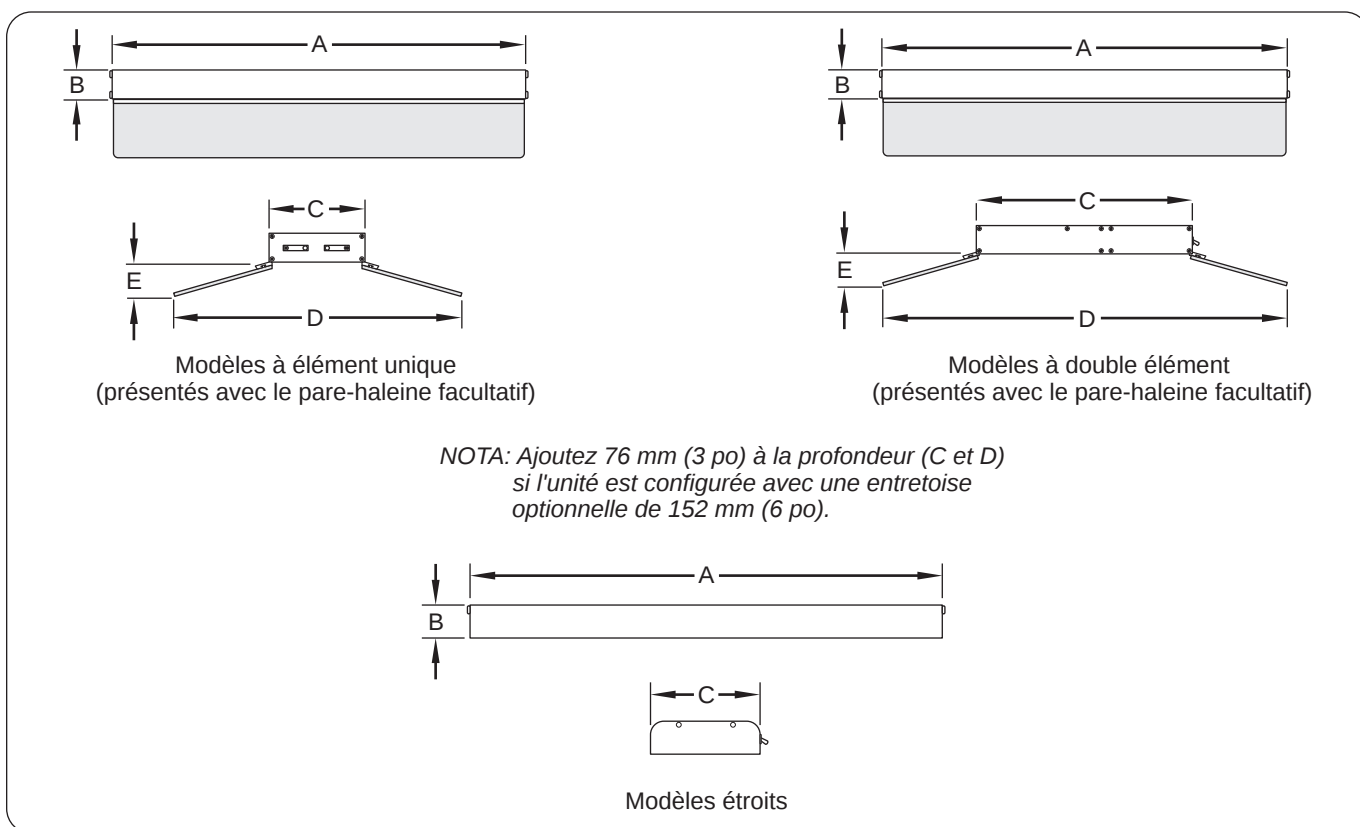
Figure 7. Dimensions
