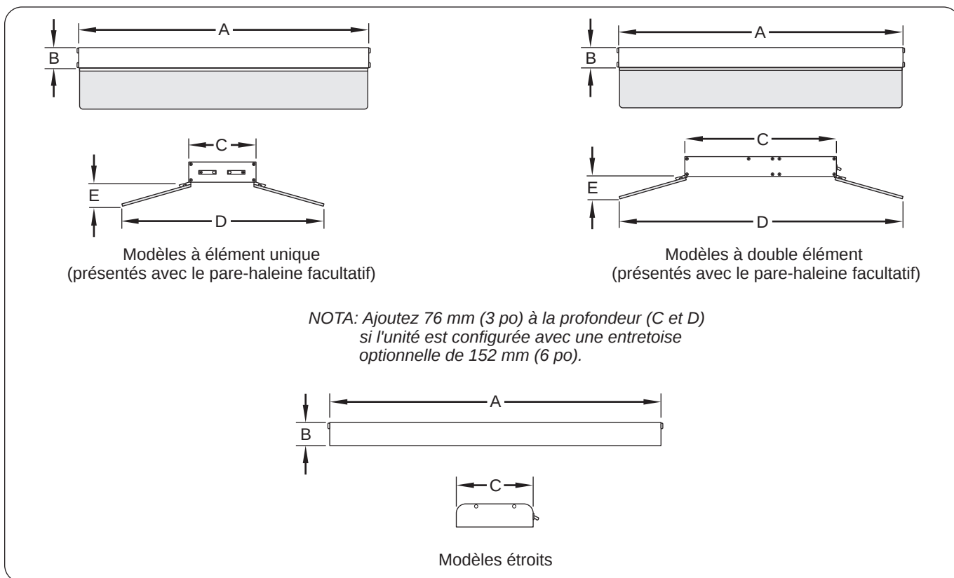
Figure 7. Dimensions
