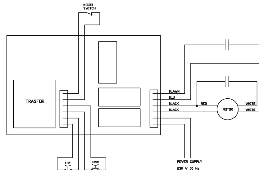
FIG. n°5 - Wiring diagram
