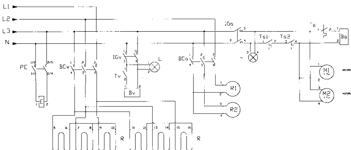
ELEMENTO BAGNOMARIA SU VANO CALDO - BAIN-MARIE UNIT IN HEATED COMPARTMENT BAINMARIE-ELEMENTE AUF BEHEIZTEM FACH – ELEMENTS BAIN-MARIE SUR COMPARTIMENT CHAUD Mod. : BC 23 (ECB 23)
