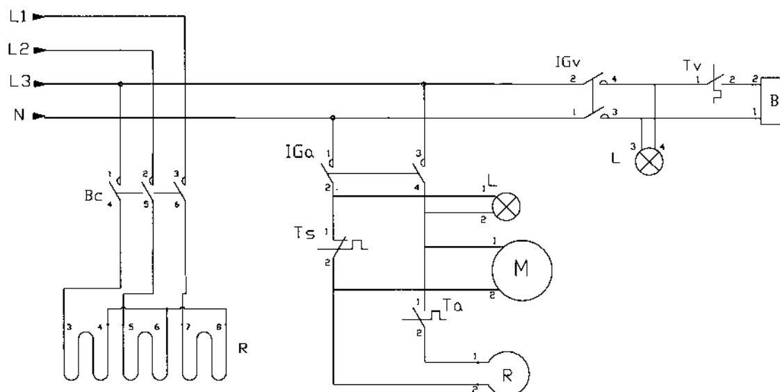
ELEMENTO BAGNOMARIA SU VANO CALDO - BAIN-MARIE UNIT IN HEATED COMPARTMENT BAINMARIE-ELEMENTE AUF BEHEIZTEM FACH – ELEMENTS BAIN-MARIE SUR COMPARTIMENT CHAUD Mod. : BC 23 (ECB 23)
