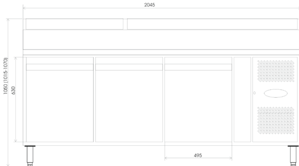
Front SS8300
