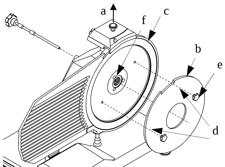
FIG. n°15 - Placing the mask in order to remove the blade
