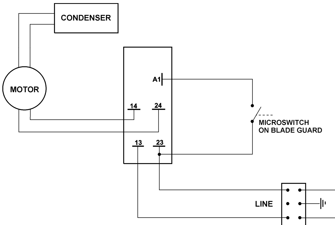
FIG. n°8 - Single-phase electric system arrangement - Schalter Profi
