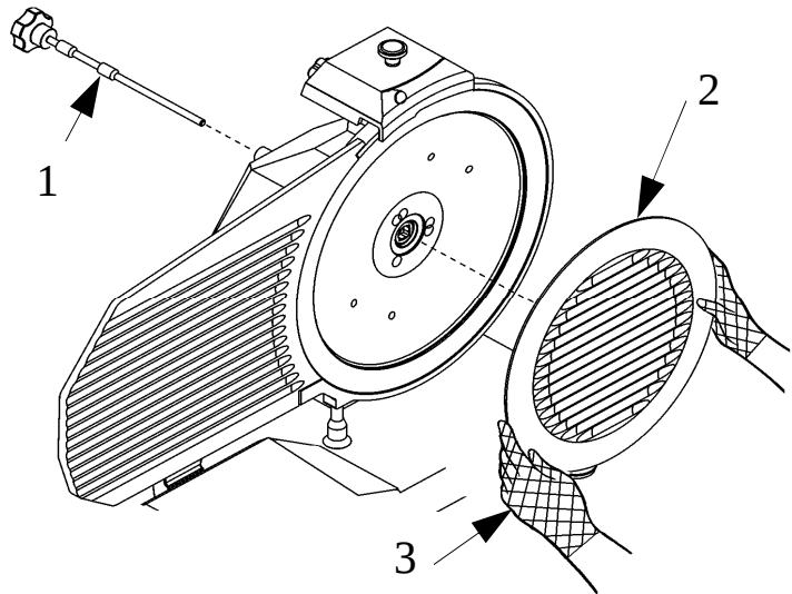
FIG. n°14 - Release of blade guard
