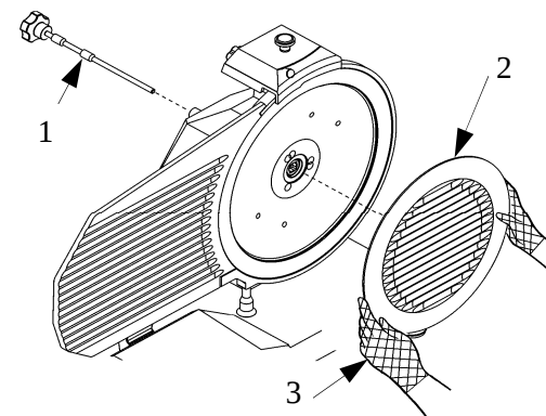
FIG. n°14 - Release of blade guard
