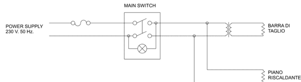
FIG. n°7 - Electrical circuit diagram of the Dispenser 51MB
