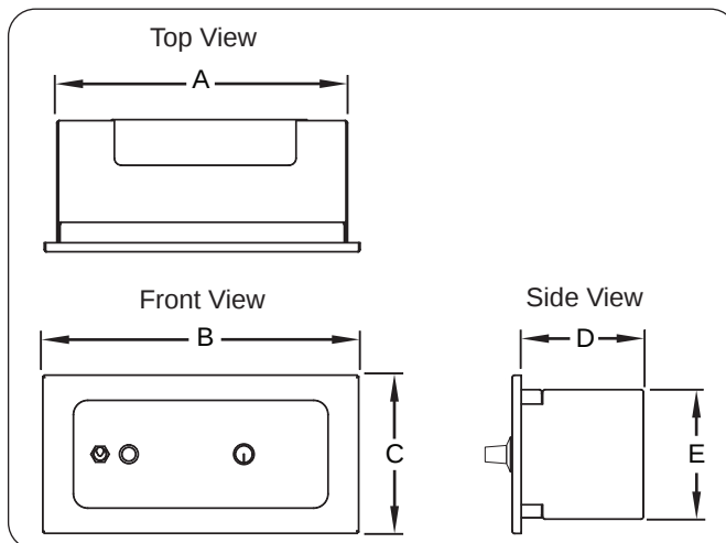
Figure 29. RMB2 Series Dimensions
