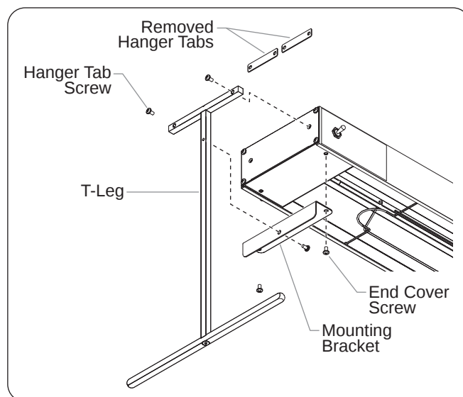
Figure 16. T-Leg Stand End Mounting
