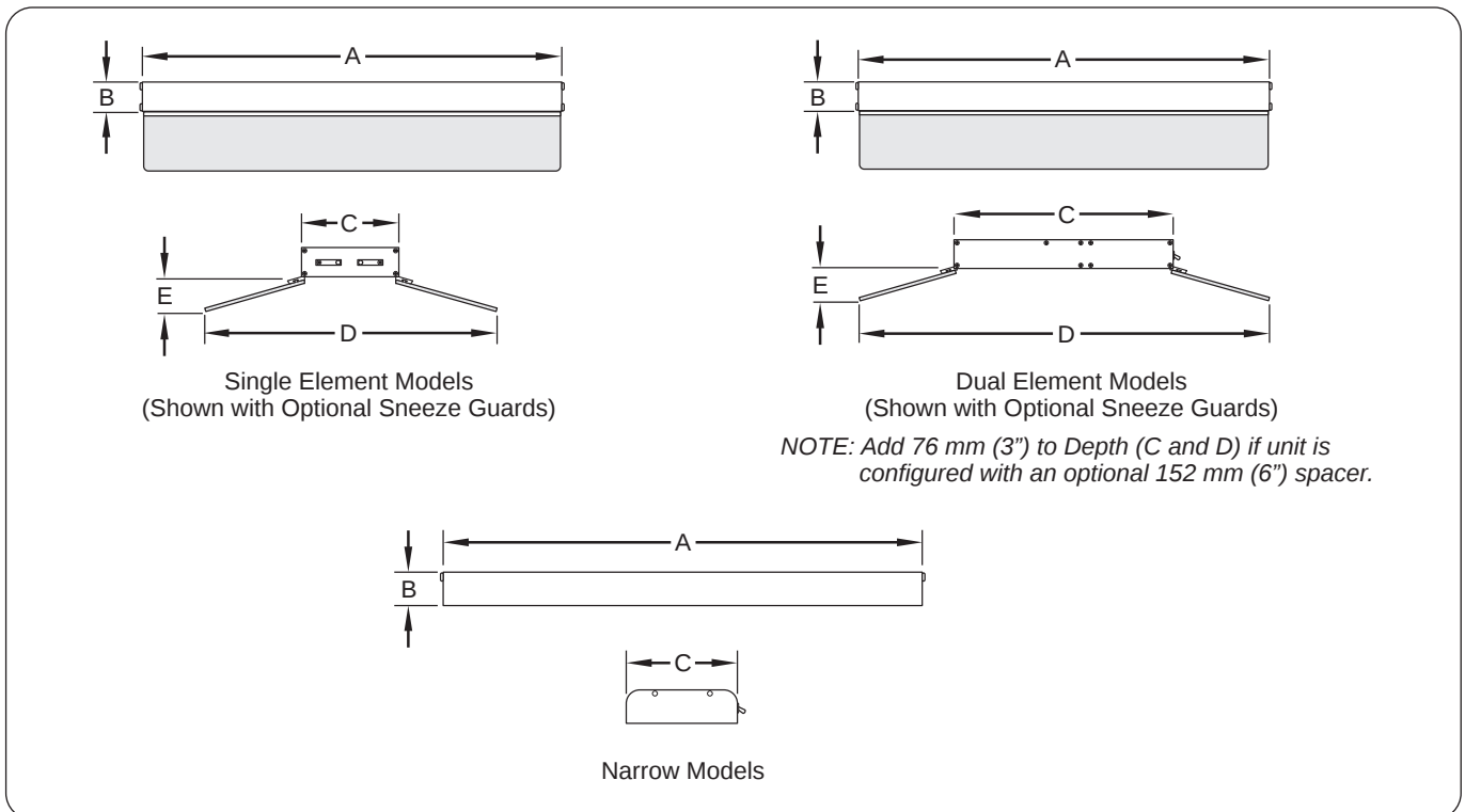
Figure 7. Dimensions
