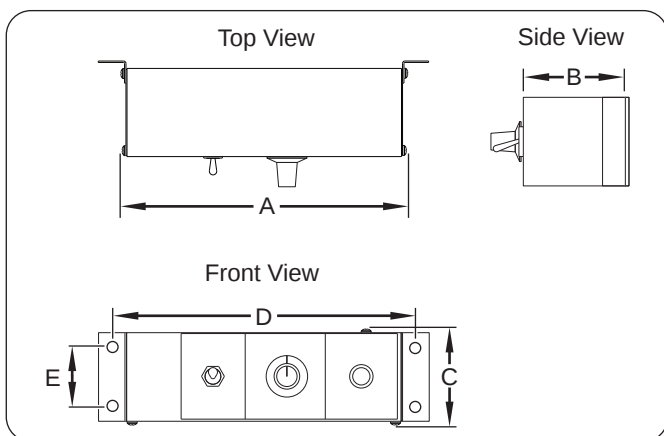
Figure 28. RMB Series Dimensions
