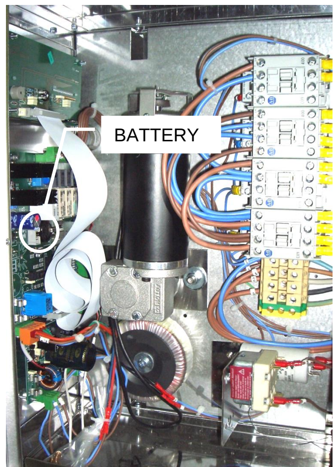
Fig. 8.1 Electronic panel, position of the BATTERY.
