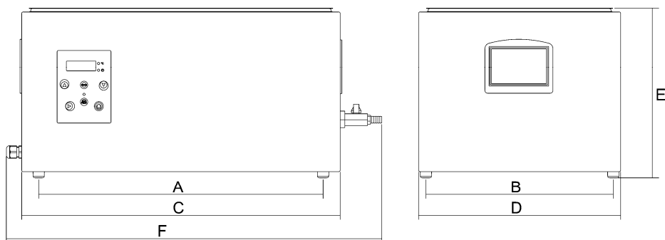
Fig.n°3 - Dimensions and max size of the machine
