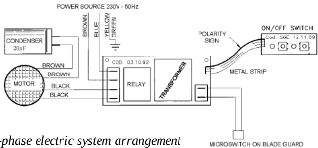
FIG. n°6 - Single-phase electric system arrangement
