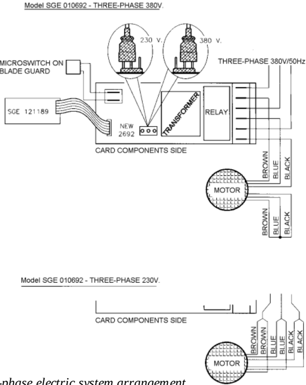
FIG. n°7 - Three-phase electric system arrangement
