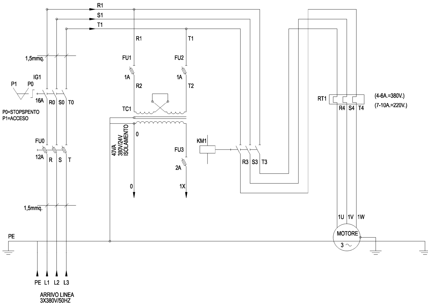
C15 2V electrical circuit diagram
