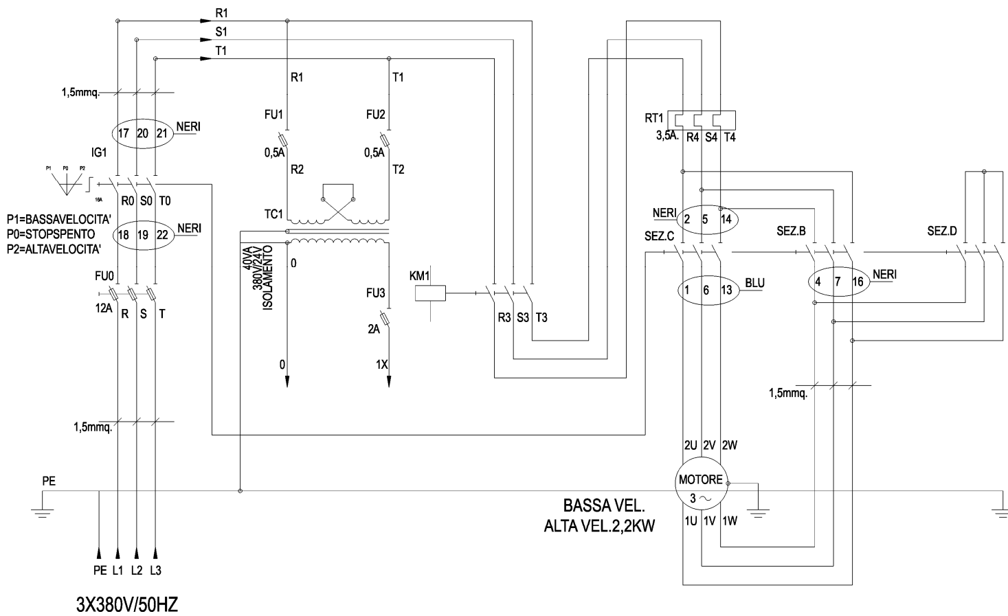
C15 2V electrical circuit diagram
