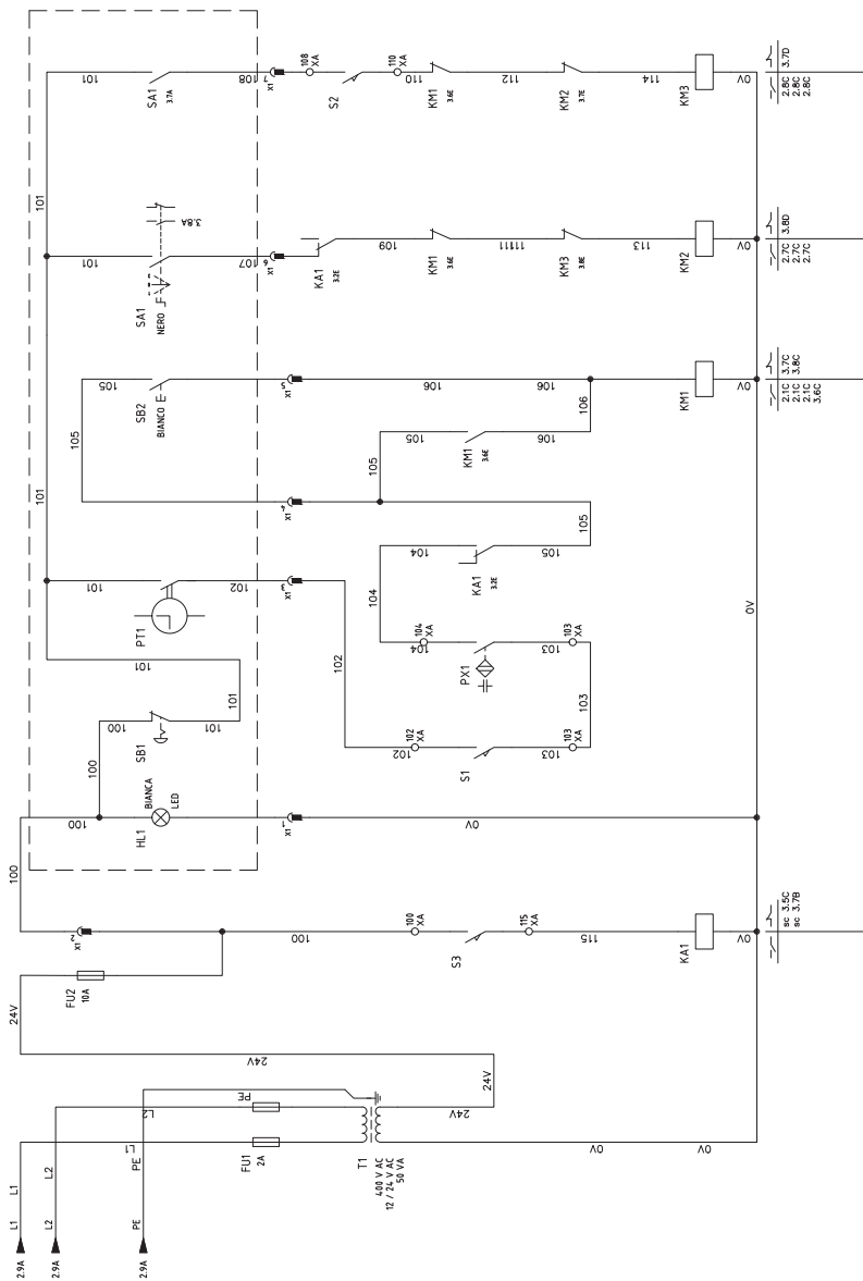
FIG. / PИC. 17 - MX40/60/80 TV
