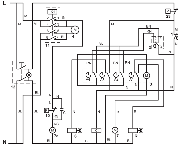
VERSIONE AD ARIA / AIR COOLED / VERSION AIRE
