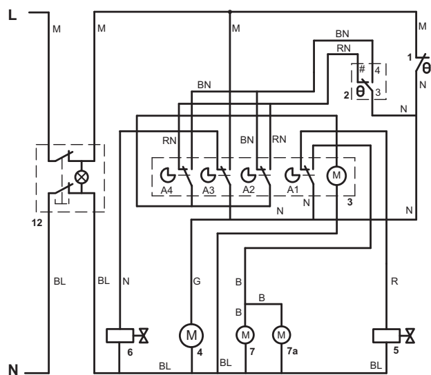
VERSIONE AD ARIA / AIR COOLED / VERSION AIRE
