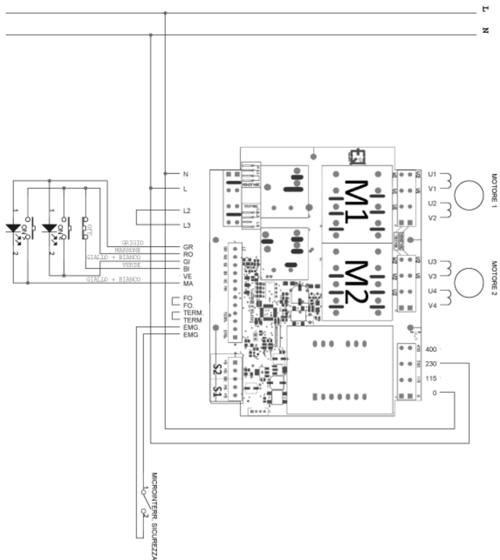
- Single-phase wiring diagram of stainless steel controls
